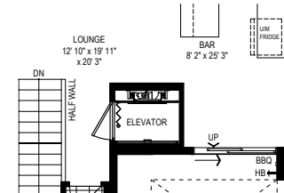
THIRD LEVEL — OPT. 1 W/ ELEVATOR
